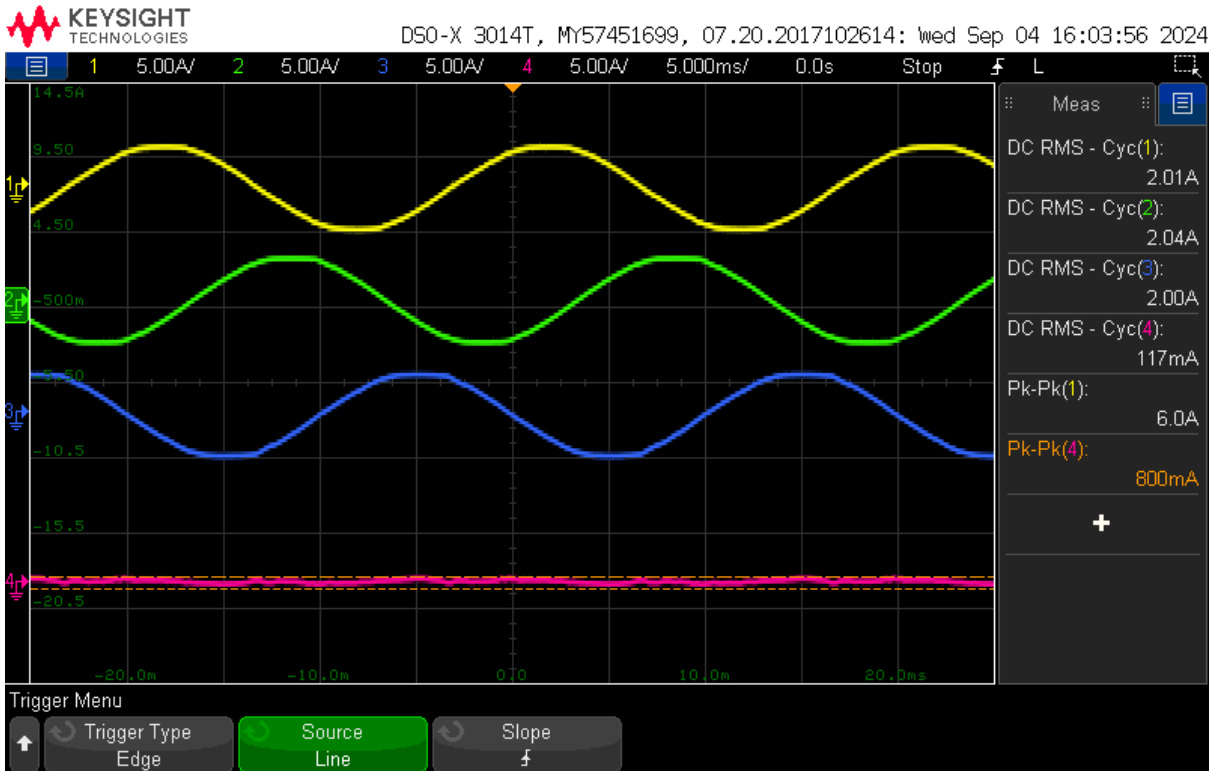
Figure 18 – MEDI MLS online UPS with APFC. Current in each phase & neutral
