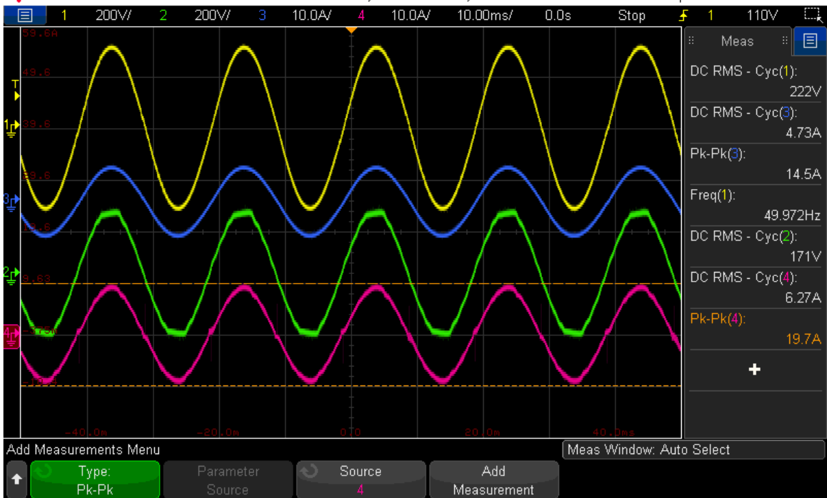
Figure 7 – Yellow output voltage, blue output current, green input voltage, red input current
